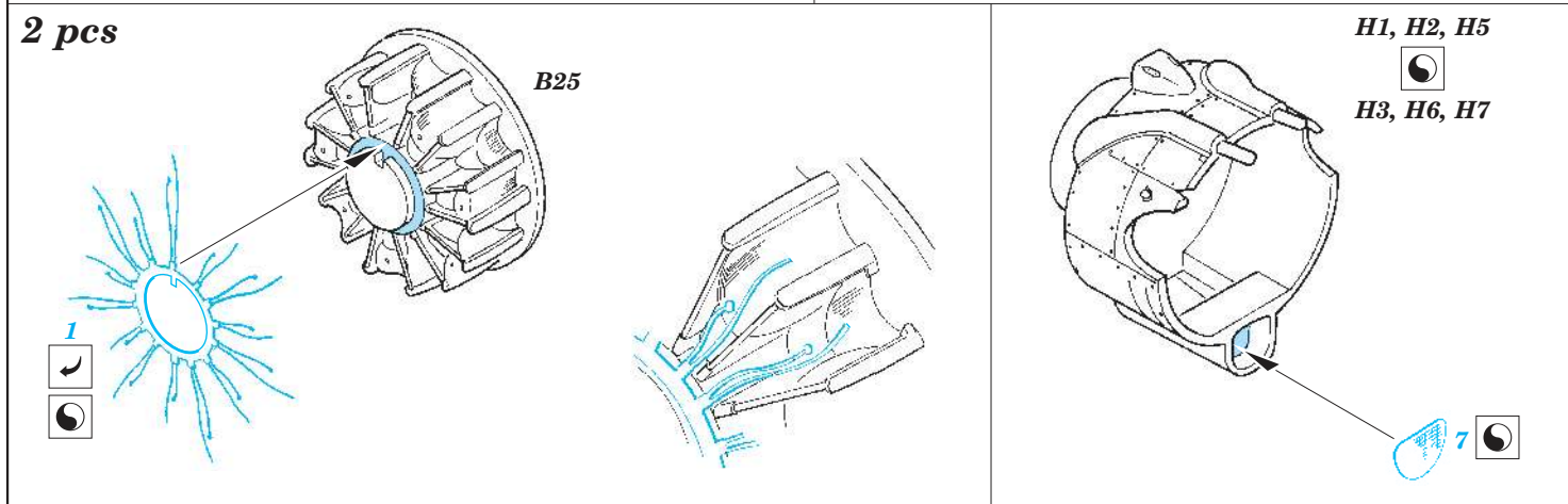
Part 67 - Left wheel well from top view
