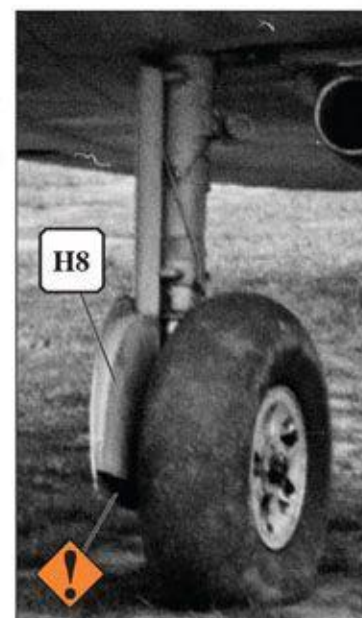
Undercarriage detail from an unidentified CBAF built 332 Squadron Spitfire Mk.Vb. Note how the wheel, strut and door are all painted the underside colour. The wide flange at the bottom of the undercarriage door is a feature mainly noted on CBAF built aircraft.
