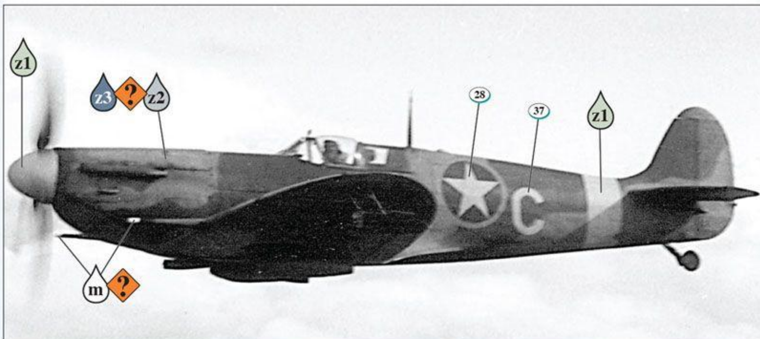
308th FS Spitfire Mk.Vb HL-C photographed in flight with Dalrymple at the controls in July 1942. Note the Roto RX5/14 propeller spinner, lack of pilot's head rest and height of the fuselage cocarde compared with the letter "C". Also note the pale linen(?) cannon muzzle covers. (E Dalrymple via Ventura Publications)
