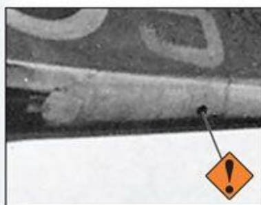
Downward firing Plessey flare device hole details from Spitfire Mk.Vb R6923 A . This was introduced into production from mid-1940.
