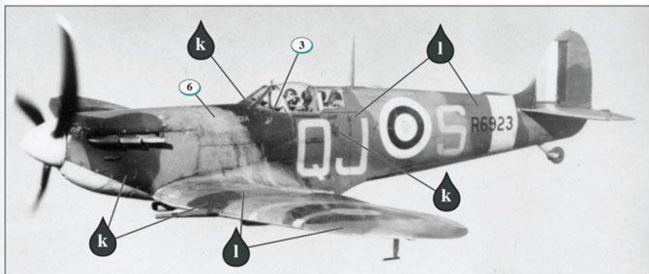
Spitfire Mk.Vb R6923. Note the heavily weathered finish and patchwork repainted areas of Dark Green. Also note the "East India Squadron" unit marking ⑥ painted on the fuel tank cover and illegible name, possibly "Sara" ③, under the windscreen. Although in this image the gun port covers appear very pale, other images confirm they are almost certainly dark red.
