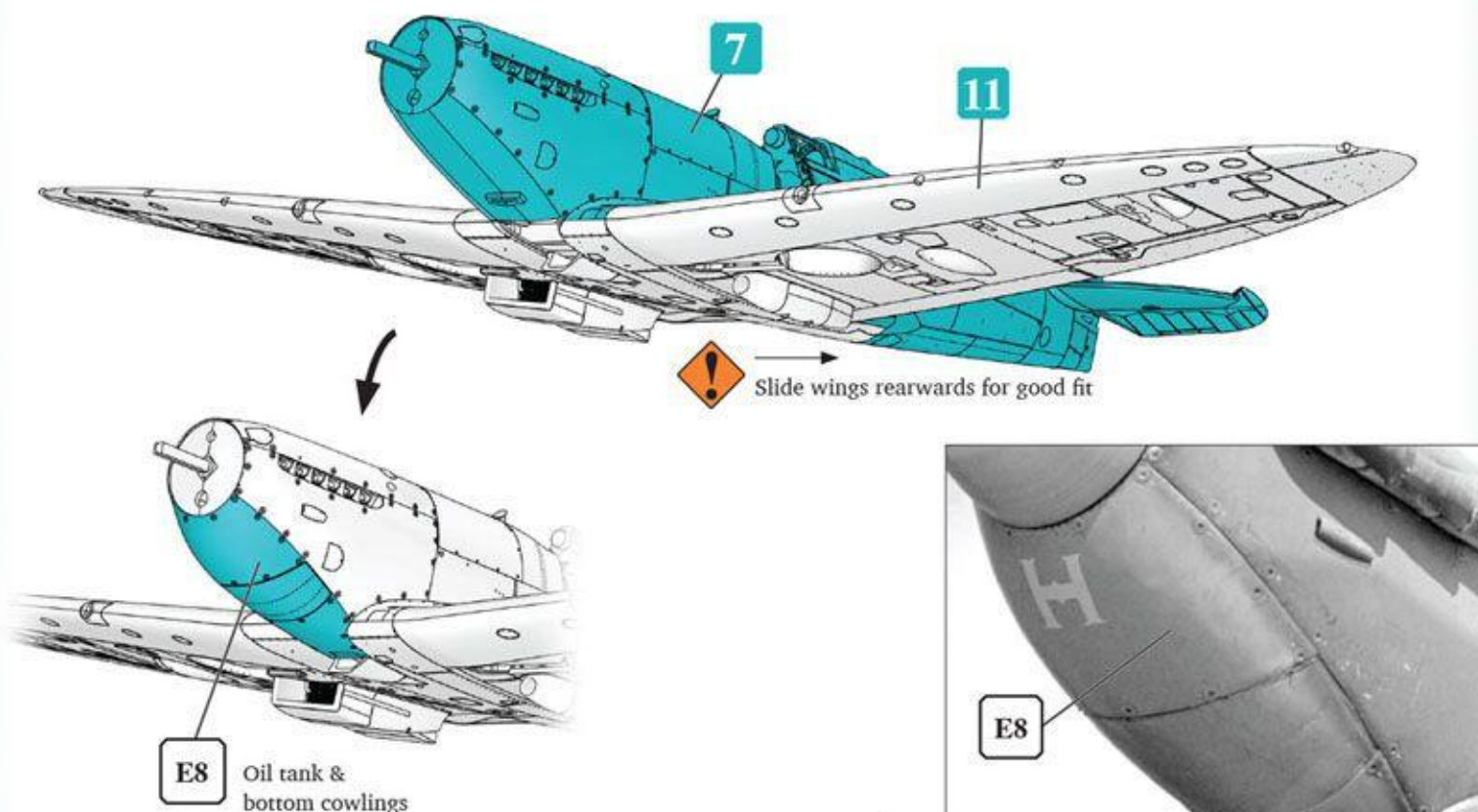
Oil tank and bottom cowlings E8 from mid-production Spitfire Mk.Vb BM202. Note the imperfect fitting panels and generally rough finish.
