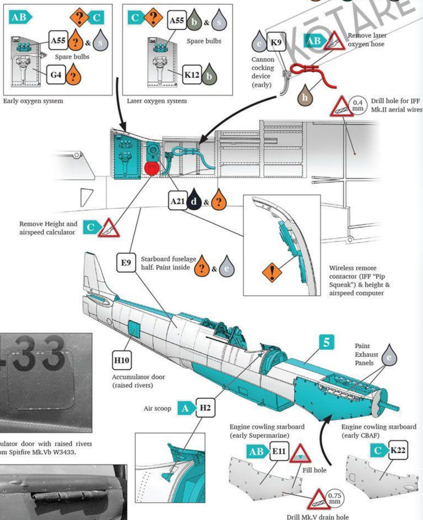
Starboard engine cowling from an early production 1440hp Merlin 45 powered CBAF built Spitfire Mk.Vb of 72 Squadron in July/August 1941. This Mk.Vb is almost certainly one of the 78 or so Mk.II completed as Mk.Vb, or 11 or so converted to Mk.Vb. Note the redundant teardrop fairing designed to clear the Coffman starter drive housing of the 1150hp Merlin XII engine of the Spitfire Mk.IIa/b. Also note the electrical engine starter plug and the key-hole for the hand crank.
