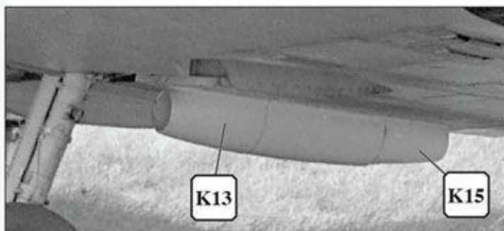
Oil cooler with full rear fairing as seen on an unidentified 54 Squadron Spitfire Mk.Va photographed in mid-1941. The lower, fully round, oil cooler opening was introduced to improve the cooling required for the more powerful Merlin 45 engine of the Mk.V.
