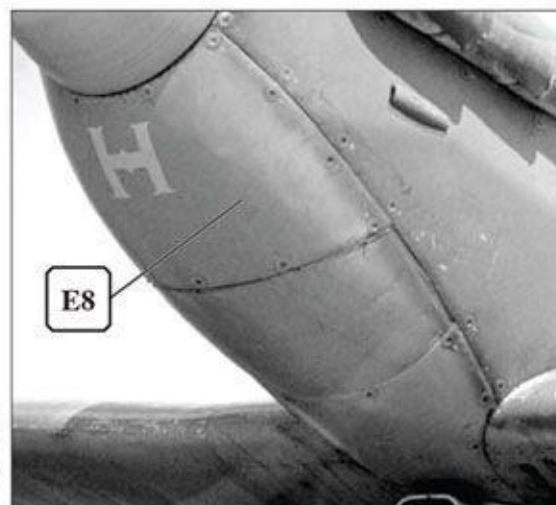
Oil tank and bottom cowlings E8 from mid-production Spitfire Mk.Vb BM202. Note the imperfect fitting panels and generally rough finish.
