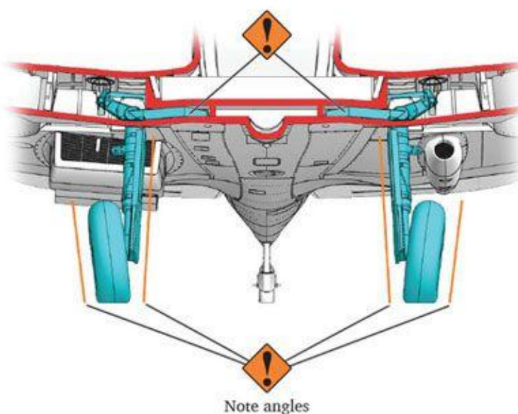
Undercarriage detail from an unidentified CBAF built 332 Squadron Spitfire Mk.Vb. Note how the wheel, strut and door are all painted the underside colour. The wide flange at the bottom of the undercarriage door is a feature mainly noted on CBAF built aircraft.
