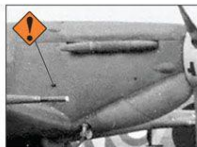
Starboard engine cowling from an early production 1440hp Merlin 45 powered CBAF built Spitfire Mk.Vb of 72 Squadron in July/August 1941. This Mk.Vb is almost certainly one of the 78 or so Mk.II completed as Mk.Vb, or 11 or so converted to Mk.Vb. Note the redundant teardrop fairing designed to clear the Coffman starter drive housing of the 1150hp Merlin XII engine of the Spitfire Mk.IIa/b. Also note the electrical engine starter plug and the key-hole for the hand crank.
